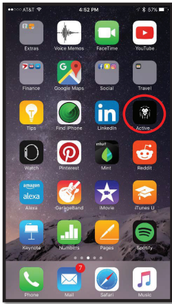
Open App
