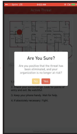
End Alert
