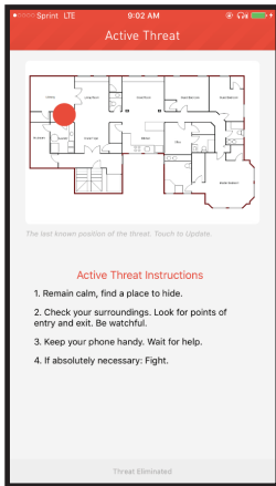
Locate Threat
