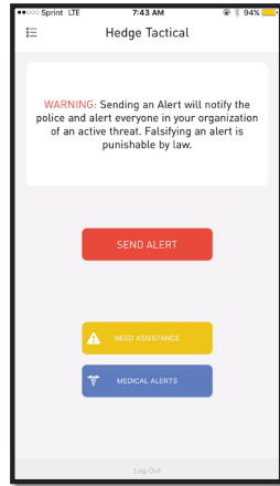
Send Alert
